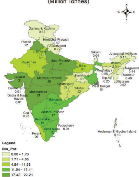
Figure 3: Surplus biomass available in India
